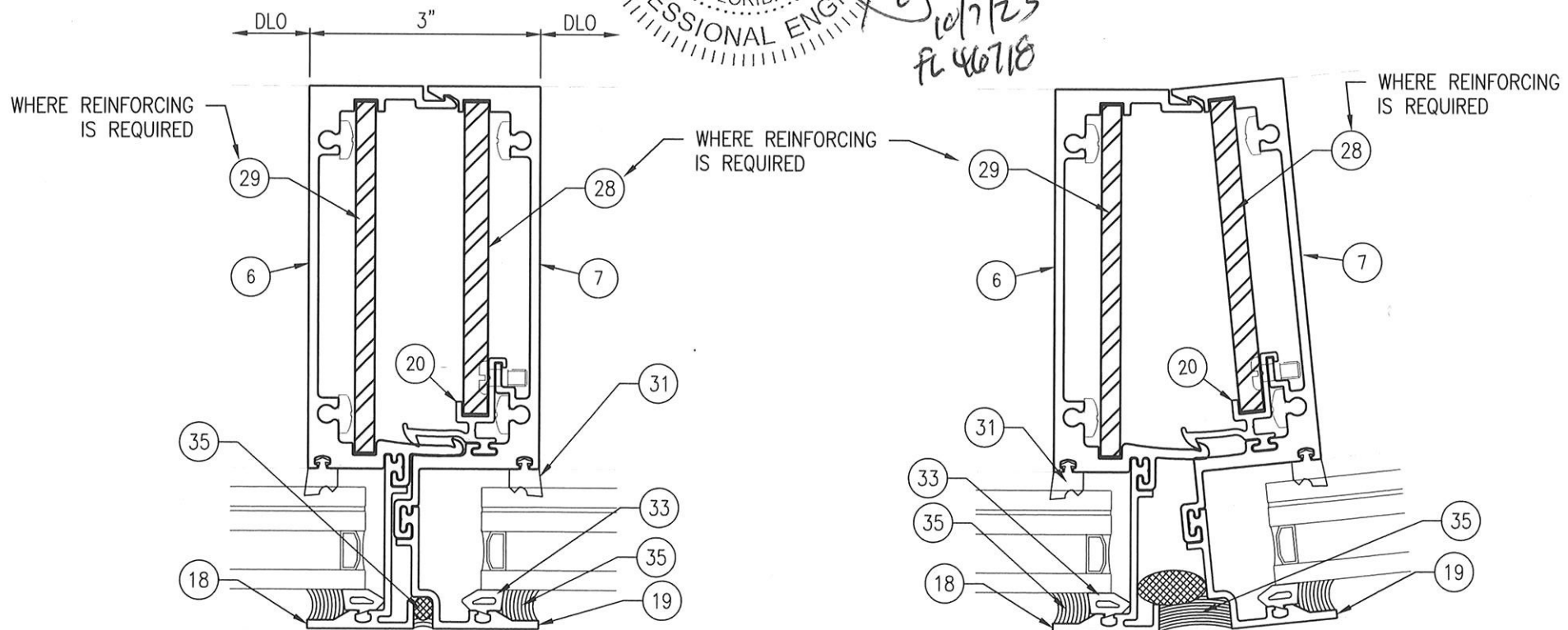
5A MULLION - CAPTURED 1-5/16" GLAZING Scale: 6" = 1'-0"
