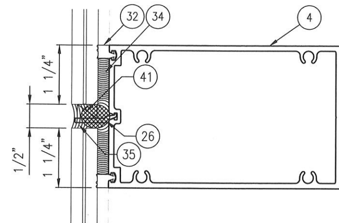
2C HORIZONTAL - BUTT GLAZED 9/16" GLAZING Scale: 6" = 1'-0"
