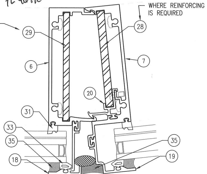
5A MULLION - CAPTURED 1-5/16" GLAZING Scale: 6" = 1'-0"
