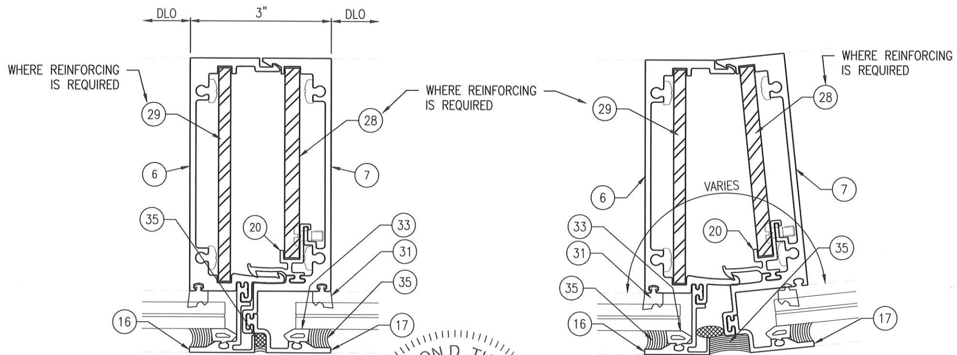
5 MULLION - CAPTURED 9/16" GLAZING Scale: 6" = 1'-0"
