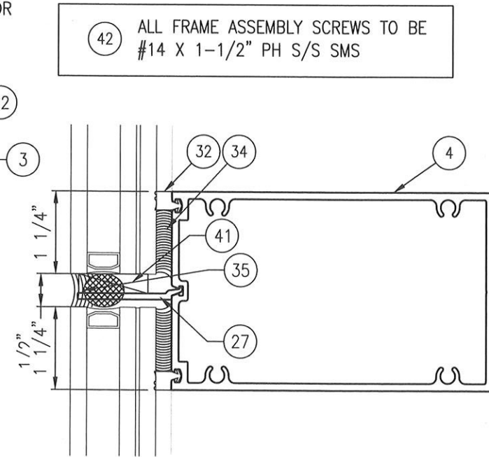
2D HORIZONTAL - BUTT GLAZED 1-5/16" GLAZING Scale: 6" = 1'-0"
